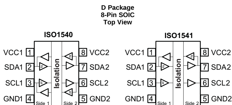
Pin Functions
